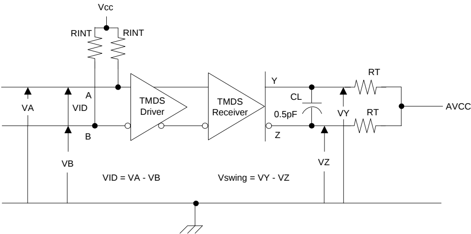
Figure 1 TMD5 Output Driver
