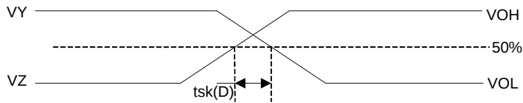
Figure 3 Definition of Intra-Pair Differential Skew
