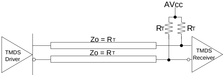
Figure 1 TMD5 Output Driver
