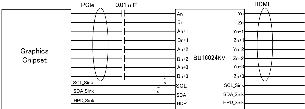
Figure 15 AC Coupling connection notice
