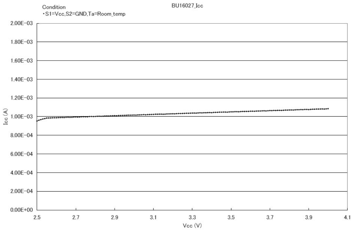
Figure 6 Supply voltage(Vcc) vs. Supply current(Icc) of BU16006KV/BU16027KV [S1=H,S2=L]
