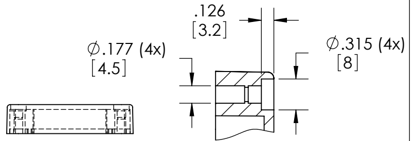
DETAIL C
