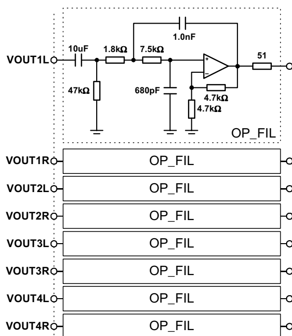
Figure 29 Recommended Post DAC Filter Circuit
