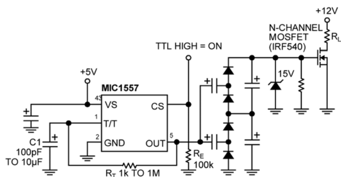
Figure 8. Charge Pump
