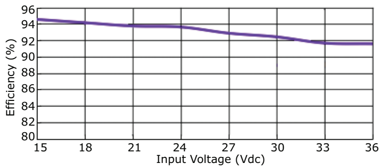
VX078012-500 Efficiency Curve Positive Output, Efficiency vs. Input Voltage (at full load)
