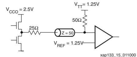
Figure 51: Terminated SSTL2 Class I
