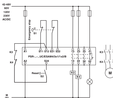
Application drawing
