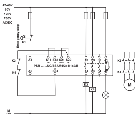
Application drawing
