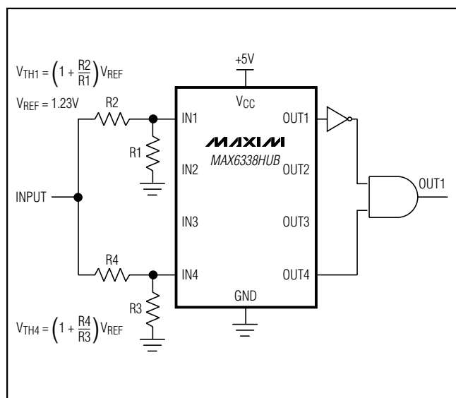
Figure 4. Window Detection
