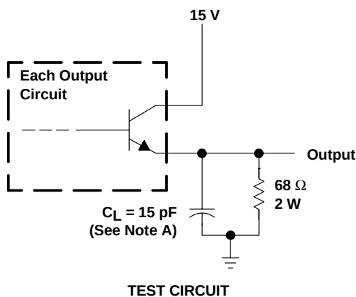
Figure 4. Emitter-Follower Configuration
