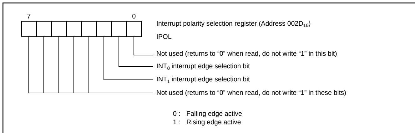
Fig. 14 Structure of interrupt polarity selection register
