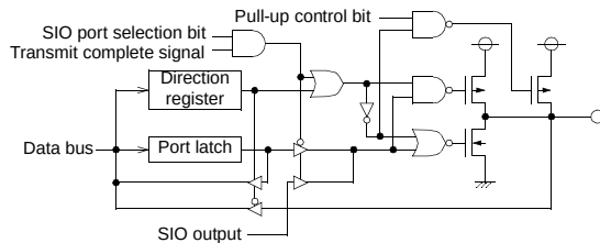
(9) Port P2 1 /S OUT
