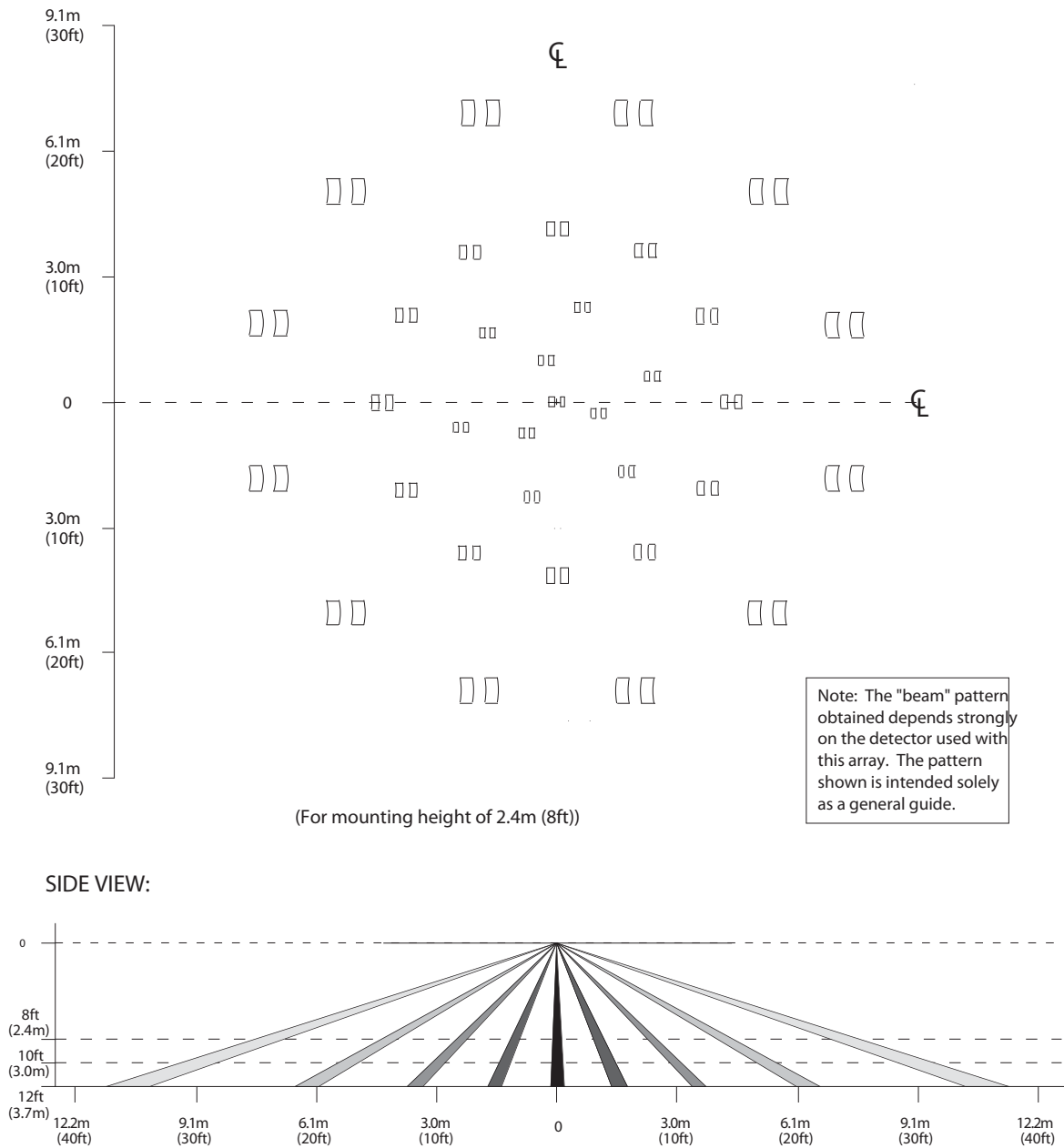
Figure 3. CM 0.77 GI V2 Lens Specification: Floor Coverage, Side View
