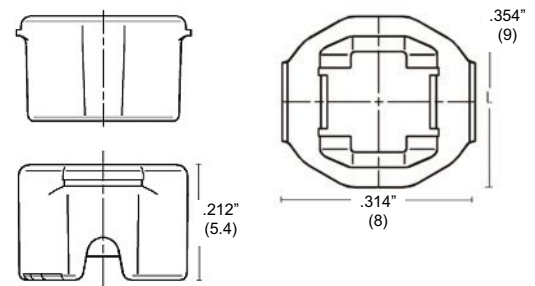
Closures ATS3080
