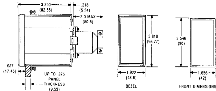
Panel Mount
