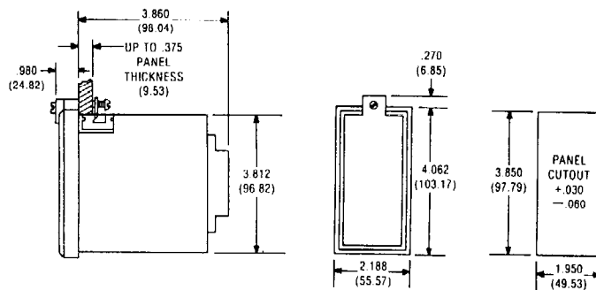
Plug-in Mount
