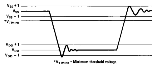
FIGURE 3. Clock Waveform
