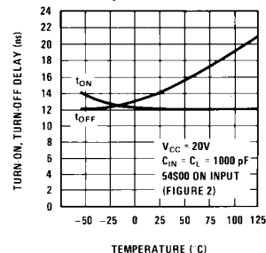
Turn-On and Turn-Off Delay vs Temperature
