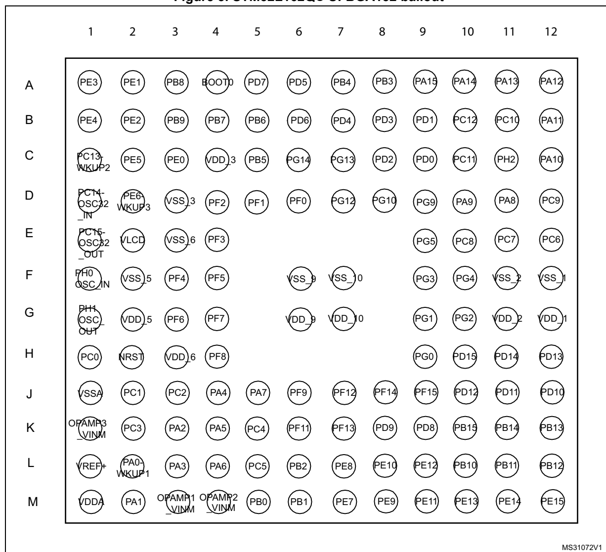
Figure 5. STM32L162QC UFBGA132 ballout
