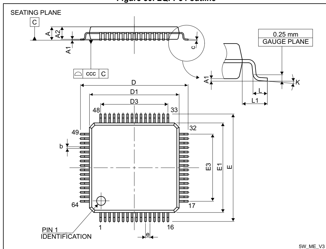
Figure 30. LQFP64 outline
