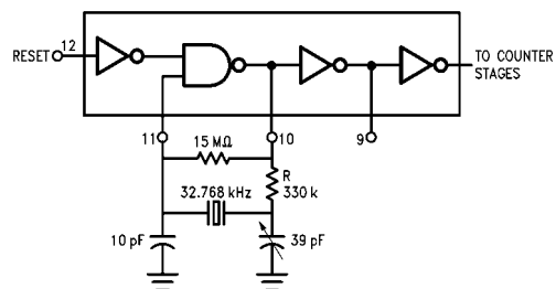
Crystal Oscillator
