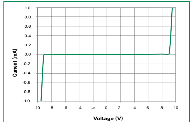
Device IV Curve - Bidirectional
