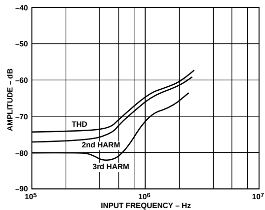
Figure 6. Distortion vs. Input Frequency, Full-Scale Input
