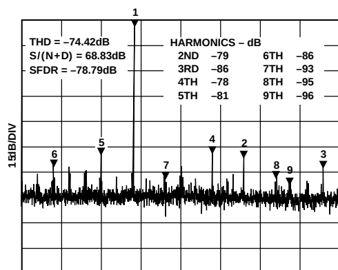
Figure 7. Typical FFT, f_{IN} = 525 kHz
