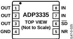
Figure 4. 8-Lead LFCSP
