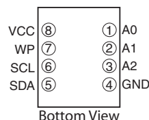
8-lead SOIC
