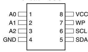
8-lead PDIP
