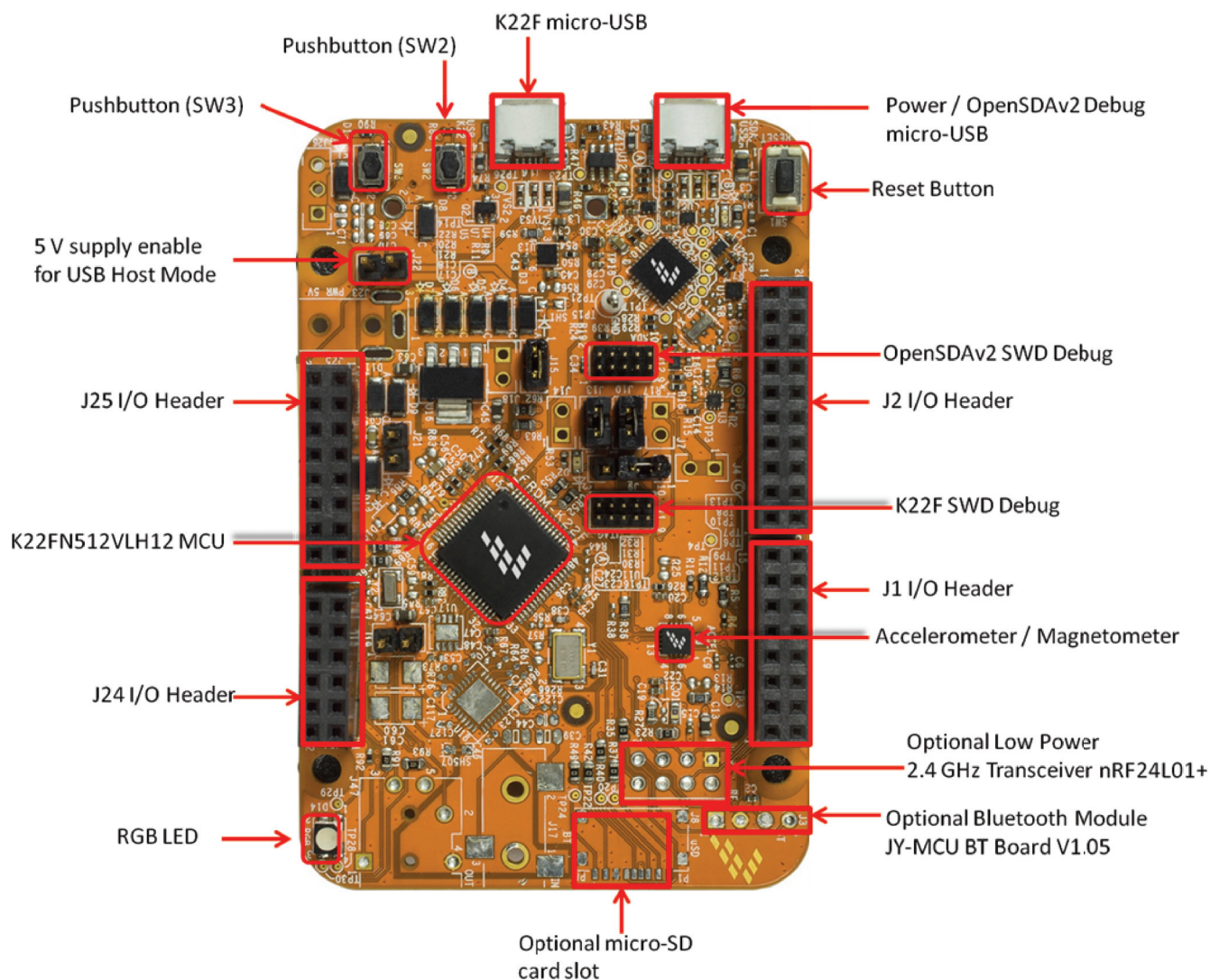
Figure 2. FRDM-K22F primary component placement
