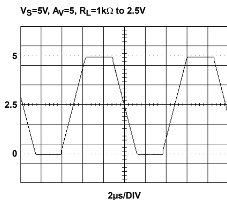
FIGURE 21. OUTPUT SWING
