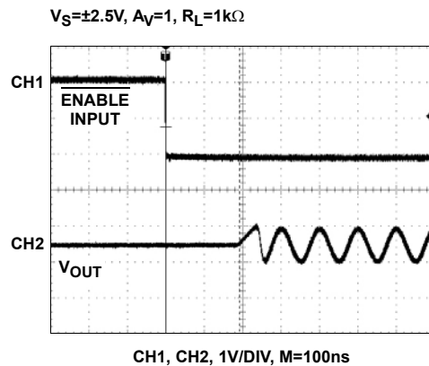
FIGURE 25. ENABLED RESPONSE
