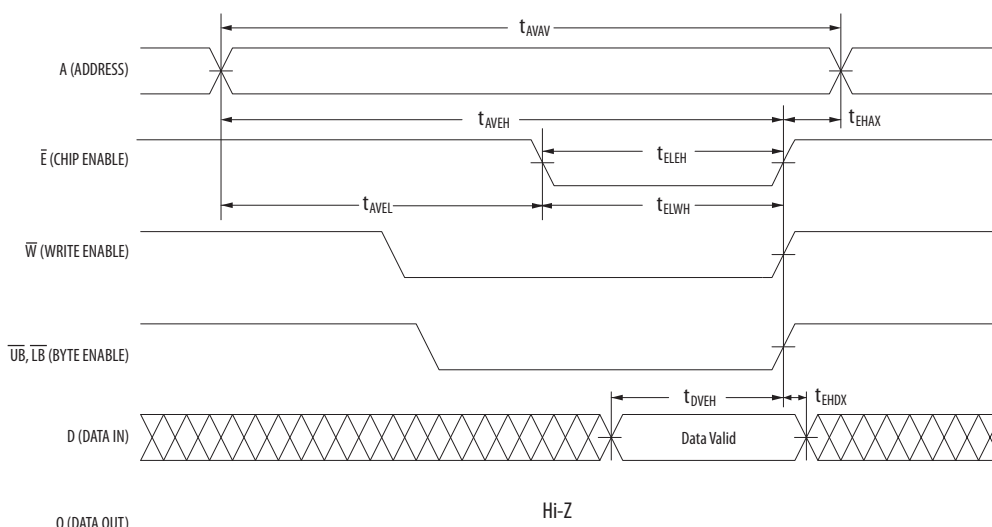
Figure 9 – Write Cycle Timing 2 ( \bar{E} Controlled)
