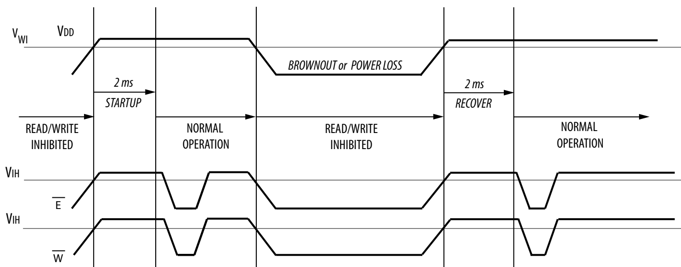
Figure 3 – Power Up and Power Down Timing
