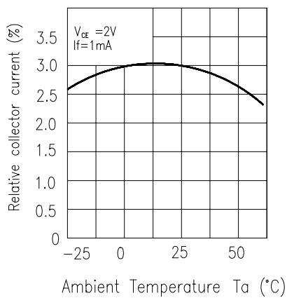
Fig. 3 Collector Current vs. Ambient Temperature
