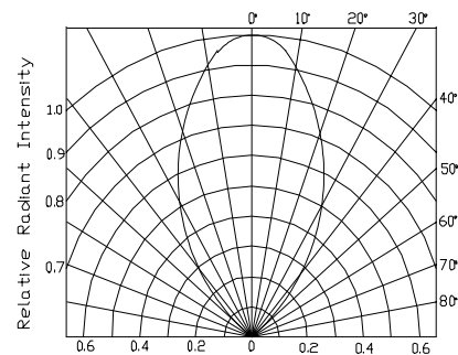
Fig. 6 Relative Radiant Intensity vs. Angular Displacement
