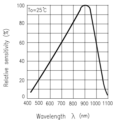
Fig.5 Spectral Sensitivity
