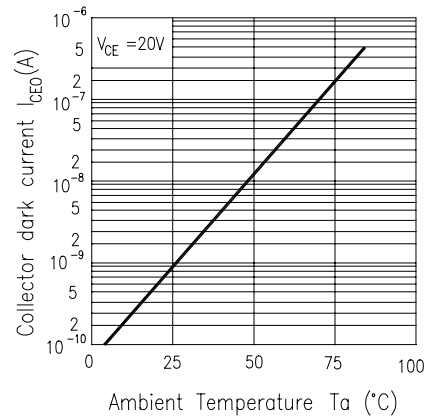
Fig.2 Collector Dark Current vs. Ambient Temperature
