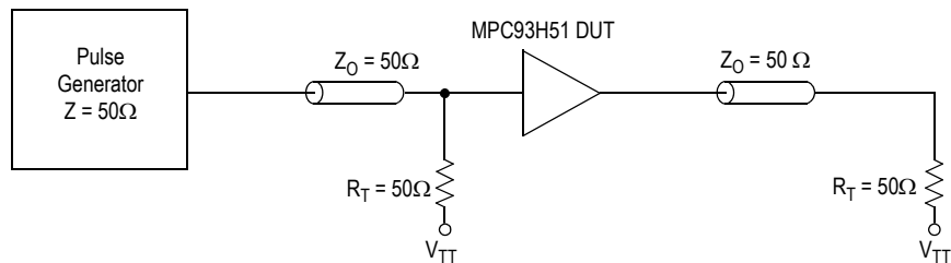
Figure 10. TCLK MPC93H51 AC Test Reference for V_{CC} = 3.3\text{ V}
