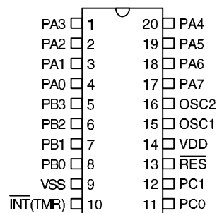
HT48C10/HT48C30 – 20 DIP-F/SOP-F
