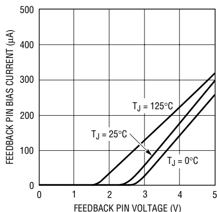
Feedback Pin Bias Current vs Feedback Pin Voltage
