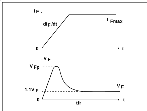
Fig. C: TURN-ON CHARACTERISTICS
