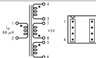
Figure 34. Coilcraft Q4339-B (Top View)
