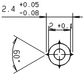
Bohrbild LP PCB-layout
