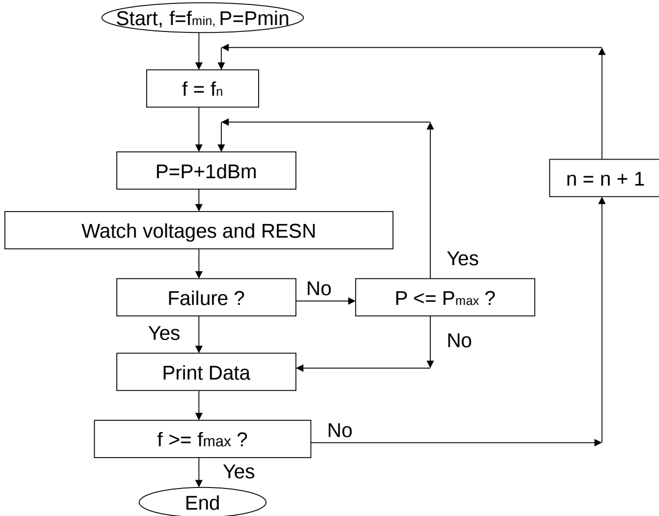
Figure 2. Test Flow
