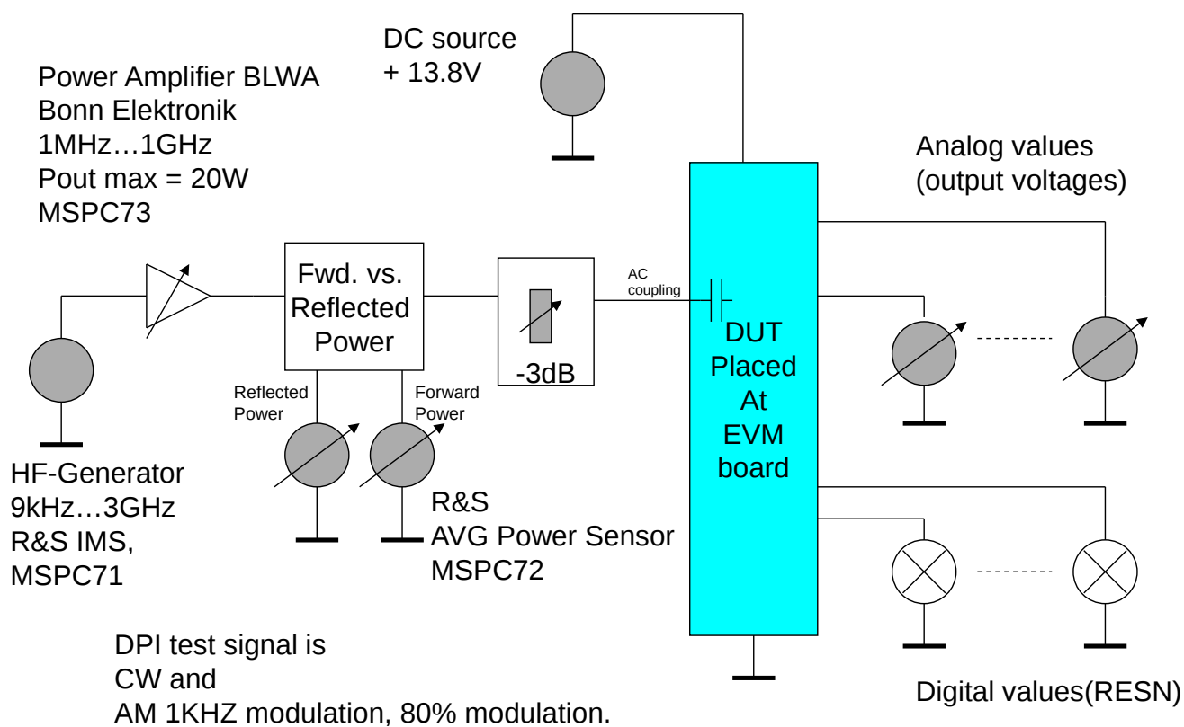
Figure 1. DPI Set Up
