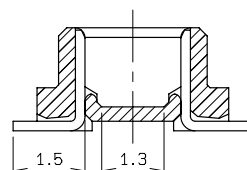
SECT. E-E
