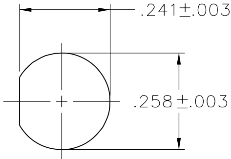
MOUNTING HOLE
