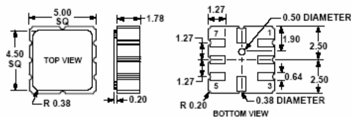
8-Terminal Ceramic Leadless Chip Carrier [LCC] (E-8)
