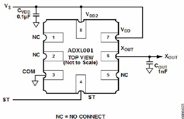
Figure 6. Application Circuit
