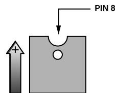
Figure 7. XOUT Increases with Acceleration in the +X-Axis Direction
