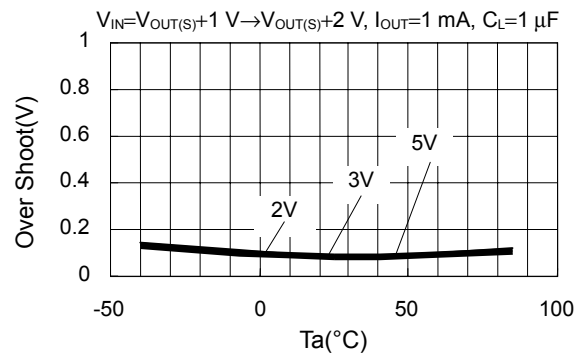
"Ta" dependencies of overshoot at power fluctuation
