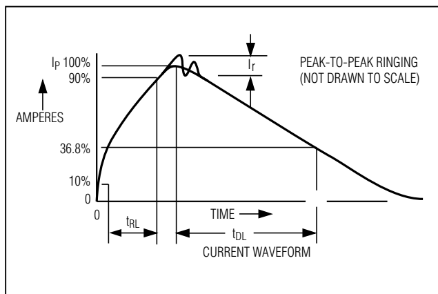
Figure 12. Human Body Model Current Waveform
