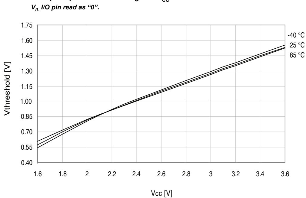
Figure 33-274. I/O pin input threshold voltage vs. V_{CC} .
