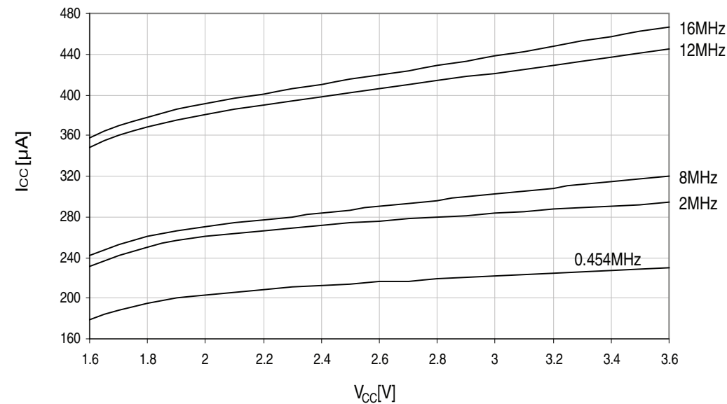
Figure 33-260. Standby supply current vs. V_{CC} . 25°C, running from different crystal oscillators.
