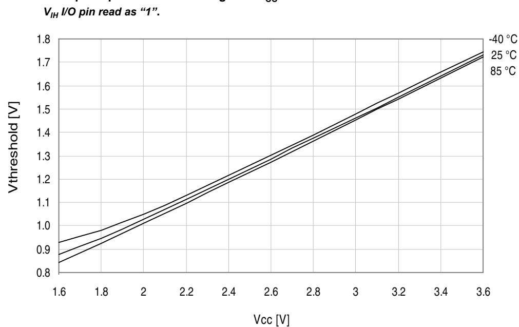
Figure 33-273. I/O pin input threshold voltage vs. V_{CC} .
