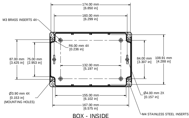
BOX - INSIDE
