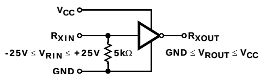
FIGURE 1. INVERTING RECEIVER CONNECTIONS
