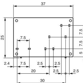
2 CO, S-Type
