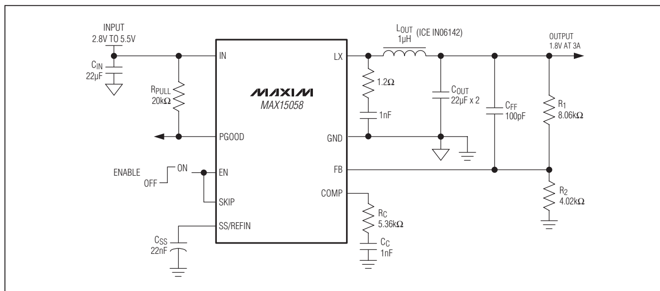
Figure 6. Application Circuit for Skip Mode Operation
