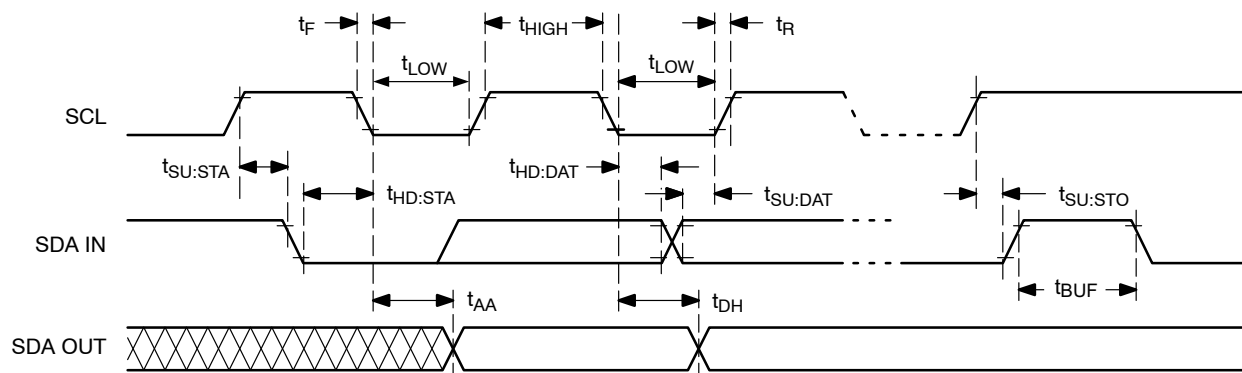
Figure 5. Bus Timing
