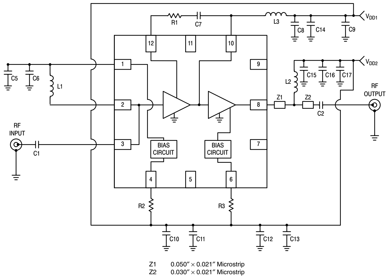
Figure 33. MML09212HT1 Test Circuit Schematic
