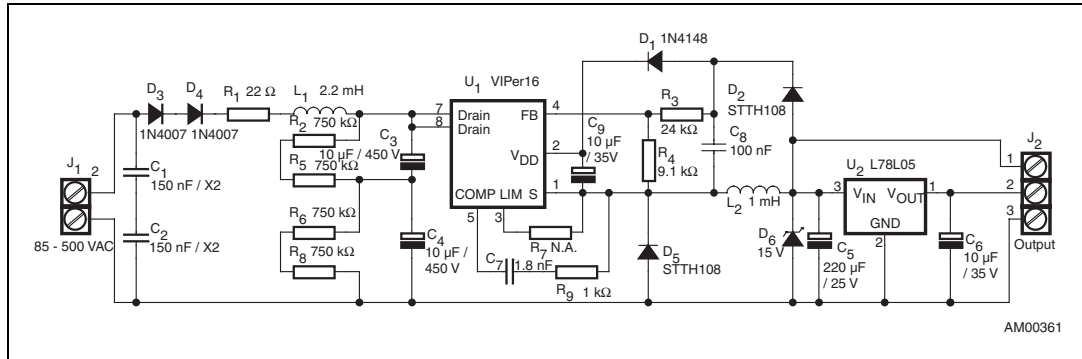
Figure 1. Schematic diagram
