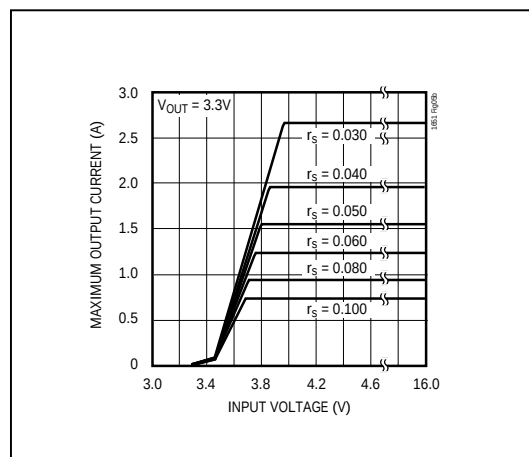
Figure 5b. MAX1651 Current-Sense Resistor Graph
