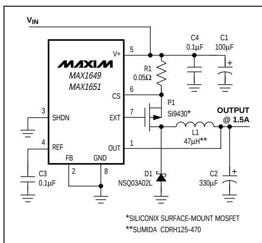
Figure 1. Test Circuit
