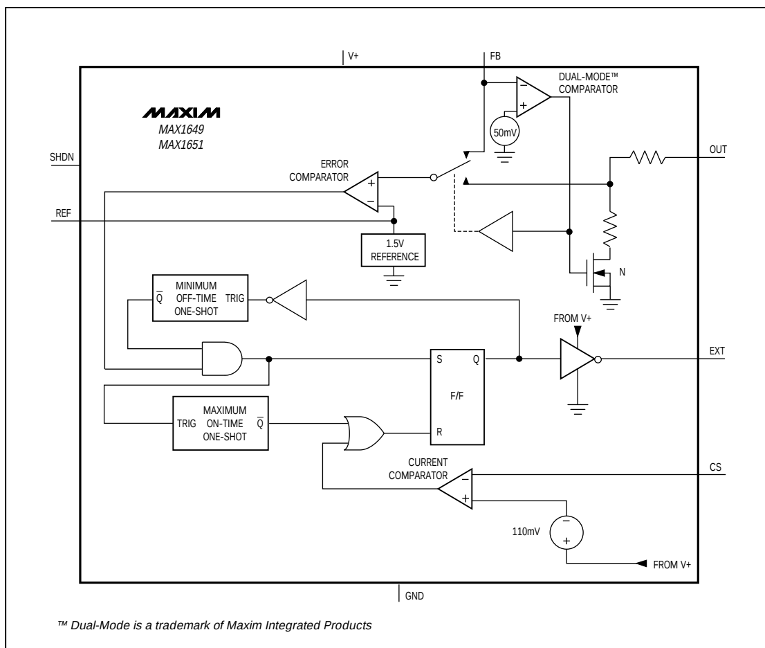
Figure 2. Block Diagram
