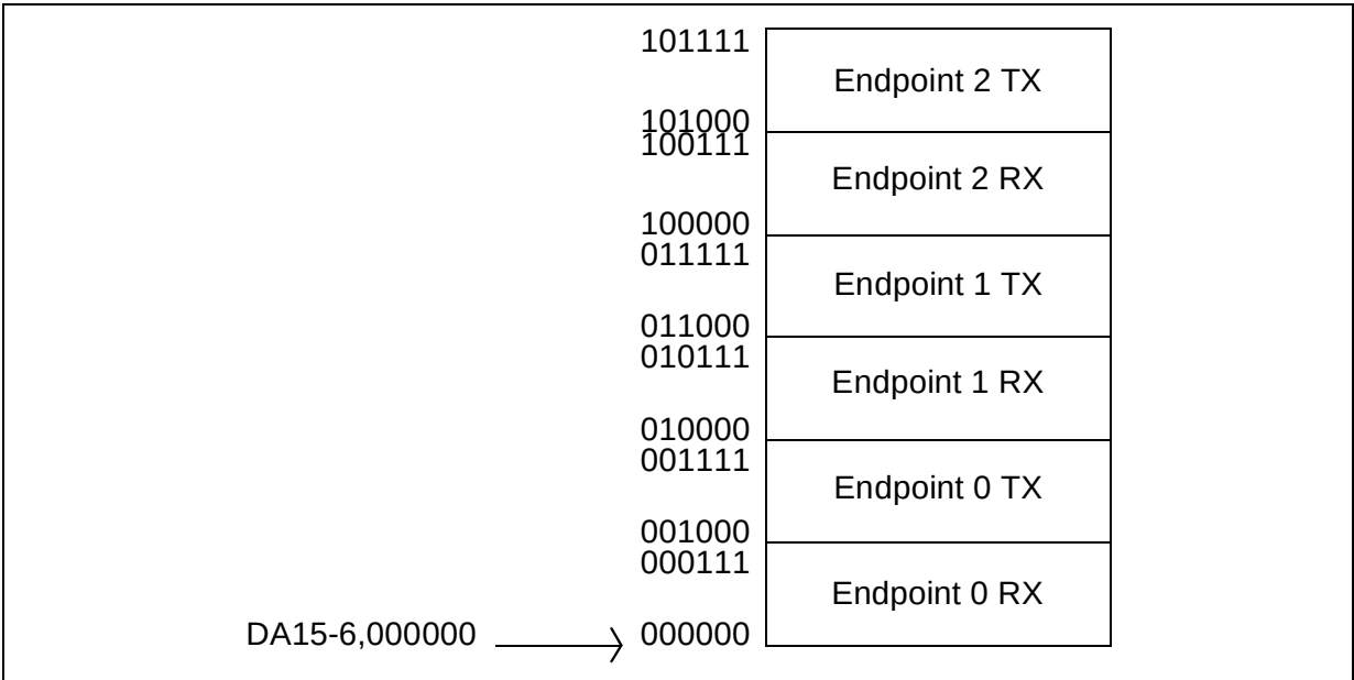
Figure 37. DMA Buffers
