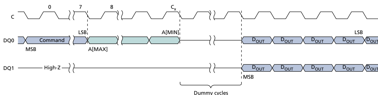
Figure 16: DUAL OUTPUT FAST READ Command Sequence
