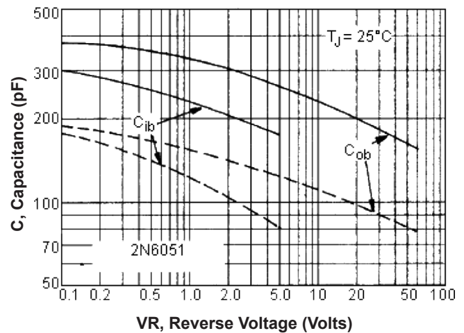
Capacitances
