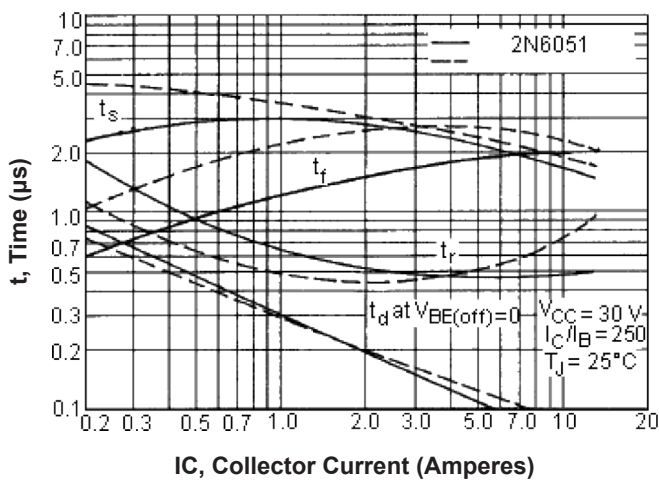
Switching Time
