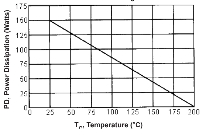
Power Derating
