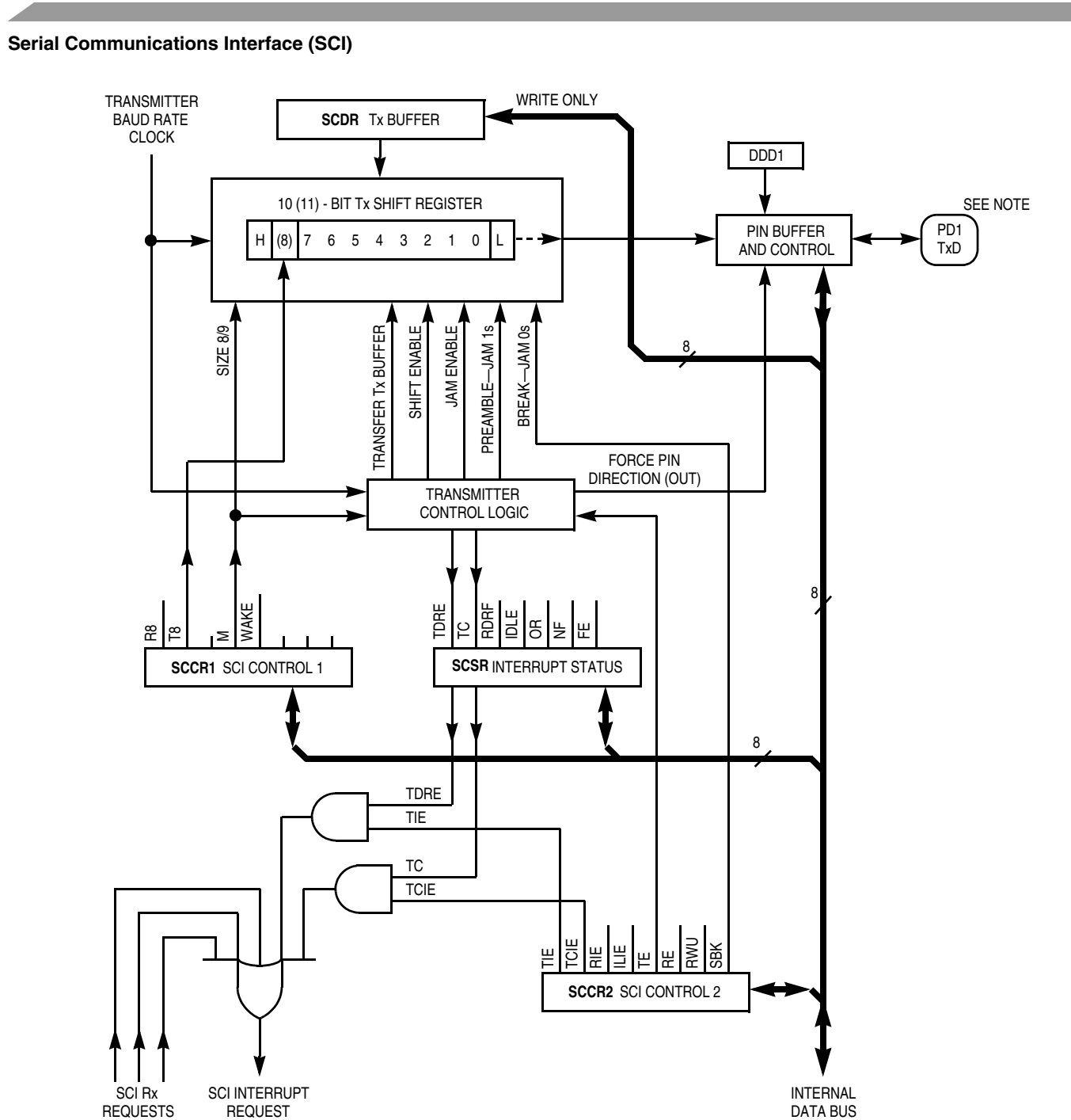
Figure 7-1. SCI Transmitter Block Diagram
