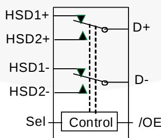
Figure 1. Analog Symbol
